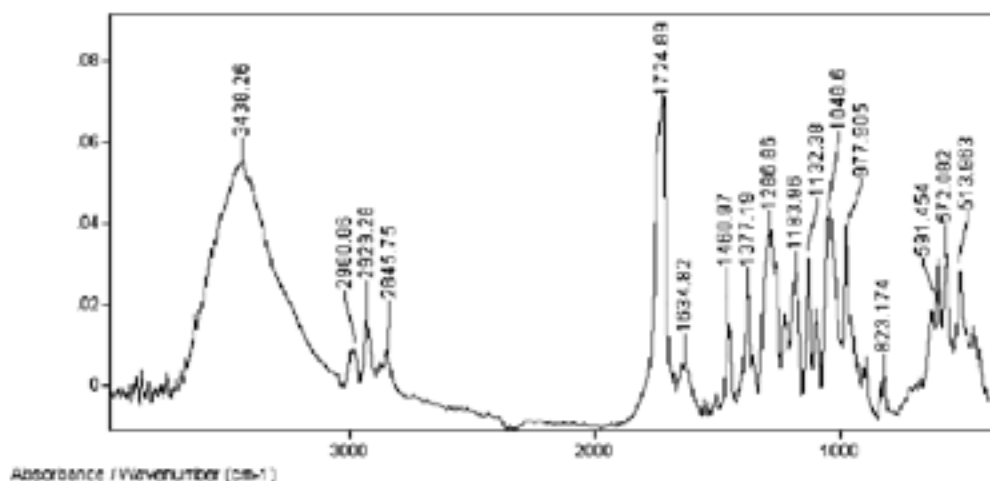
Figure 1. FTIR absorption spectrum of PHB.
